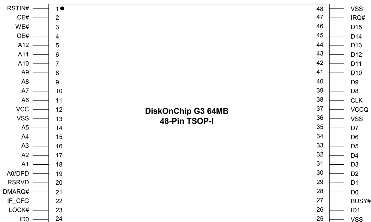
Figure 1: TSOP-I Pinout for Standard Interface (DiskOnChip G3 64MB/512Mb)
