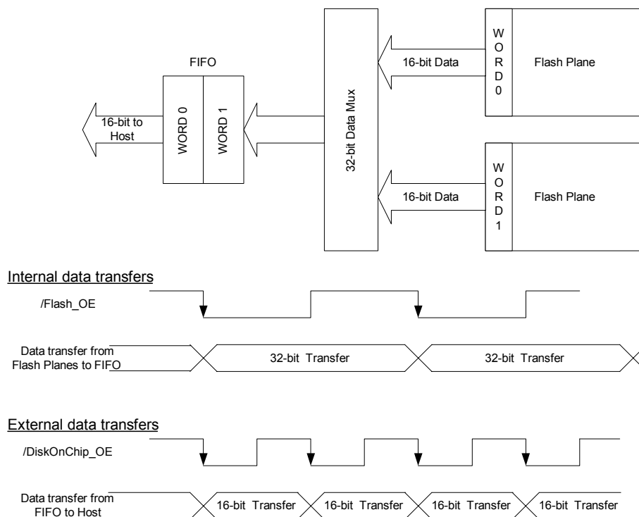
Figure 15: MultiBurst Operation
